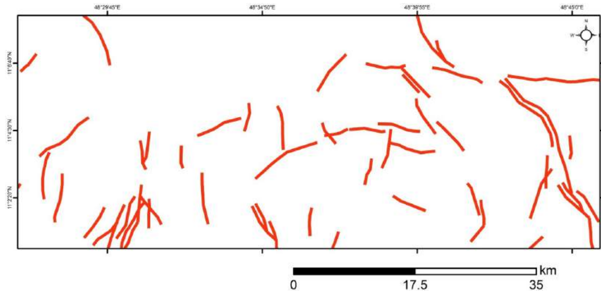
Fig. 7 Surface Lineament Map of the Study Area
