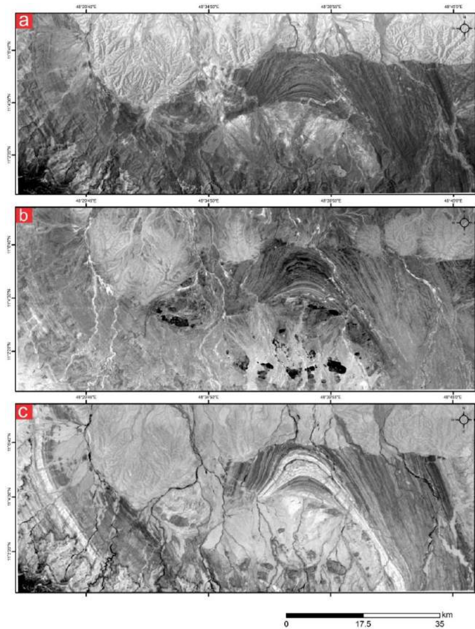
Fig. 5 Band ratio grayscale images: (a) B4/B2 highlighting iron oxides; (b) B6/B7 emphasizing hydroxyl and carbonate minerals; (c) B6/B5 enhancing ferrous minerals.
