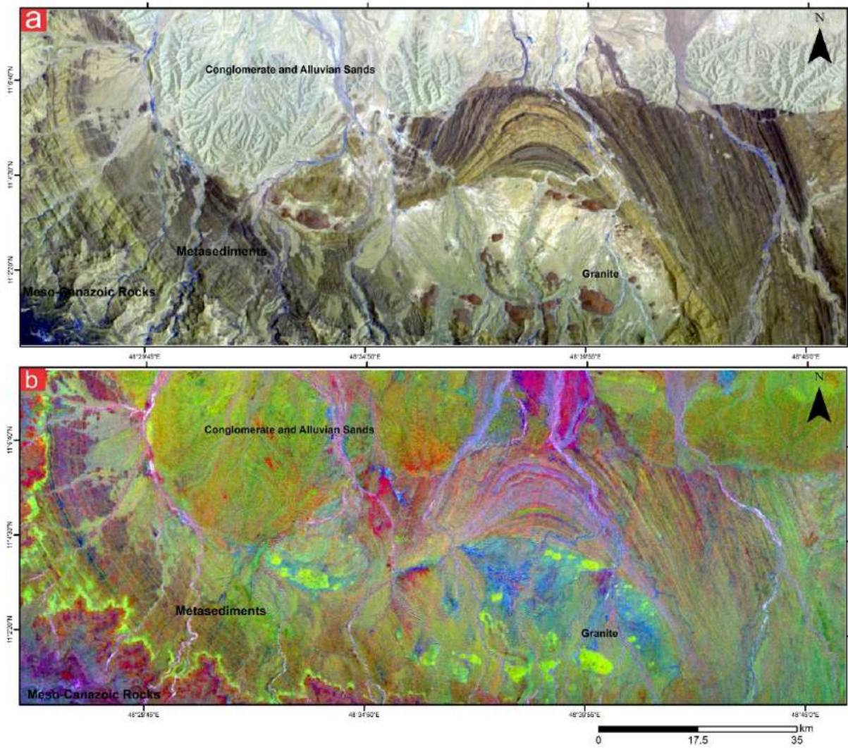
Fig. 4 RGB image combinations used for lithological interpretation: (a) 7-6-5 (RGB) false-color composite; (b) Principal Component Analysis (PCA) image displayed using a 6-5-7 (RGB) band combination.
