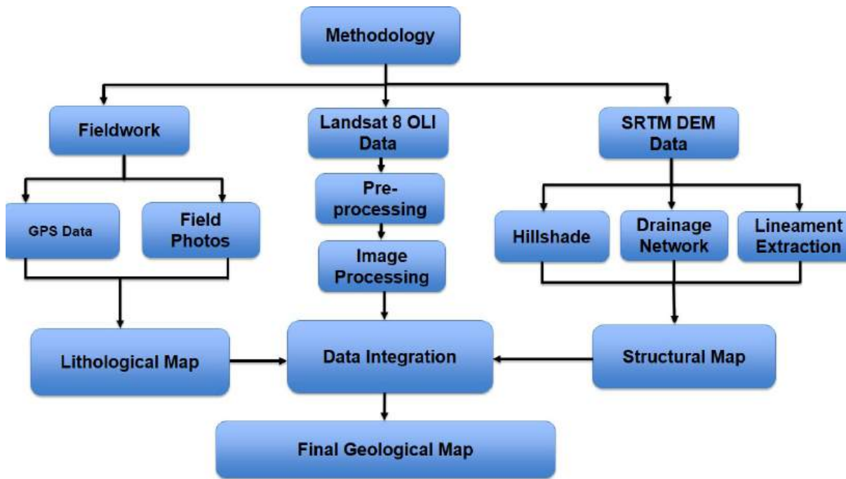
Fig. 3 Flowchart of the adopted methodology
