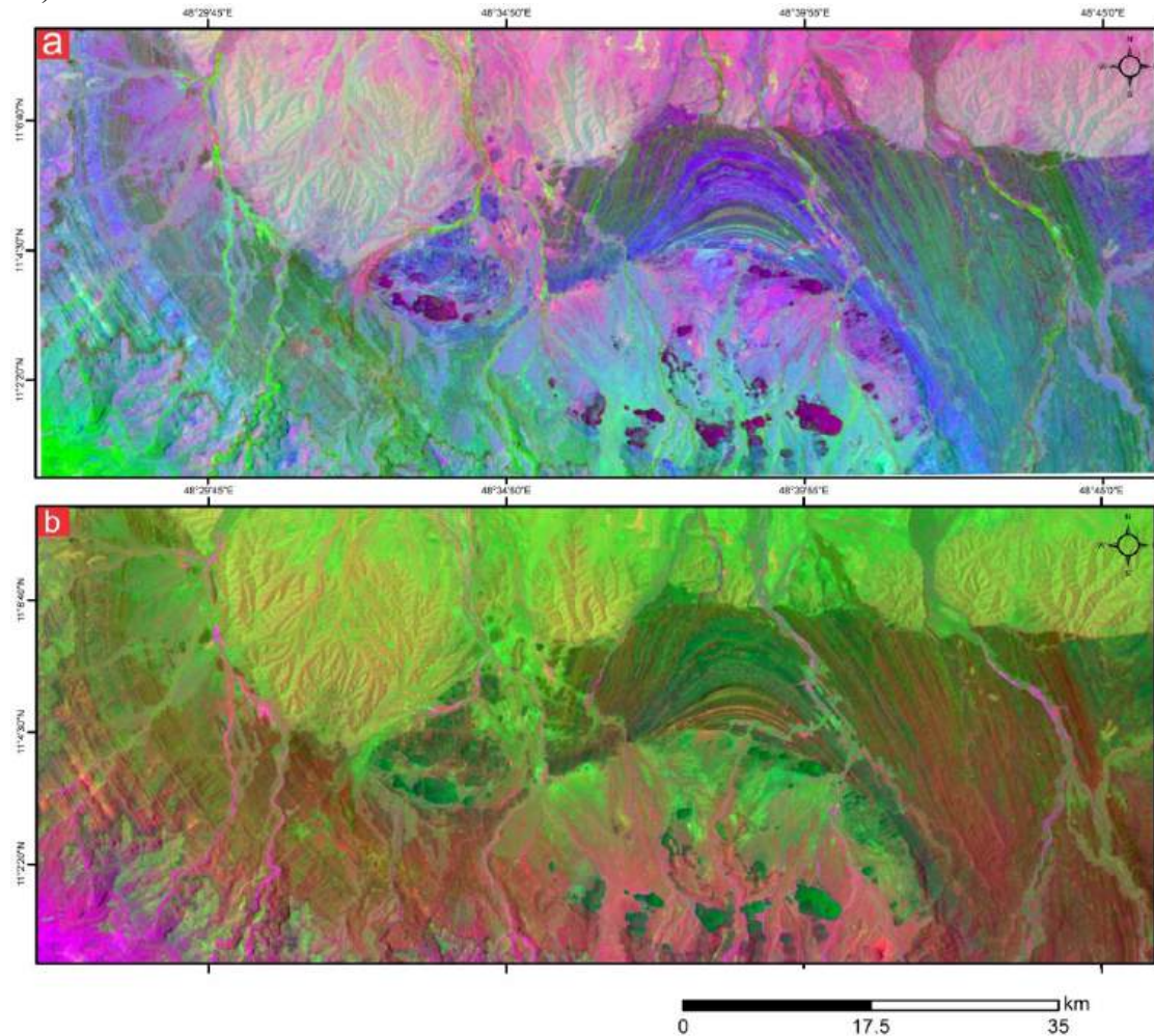
Fig. 6 RGB composite band ratios for hydrothermal alteration mapping: (a) Sabin's ratio using 4/2, 6/7, 6/5 (RGB); (b) Kaufmann ratio using 7/5, 5/4, 6/7 (RGB).
