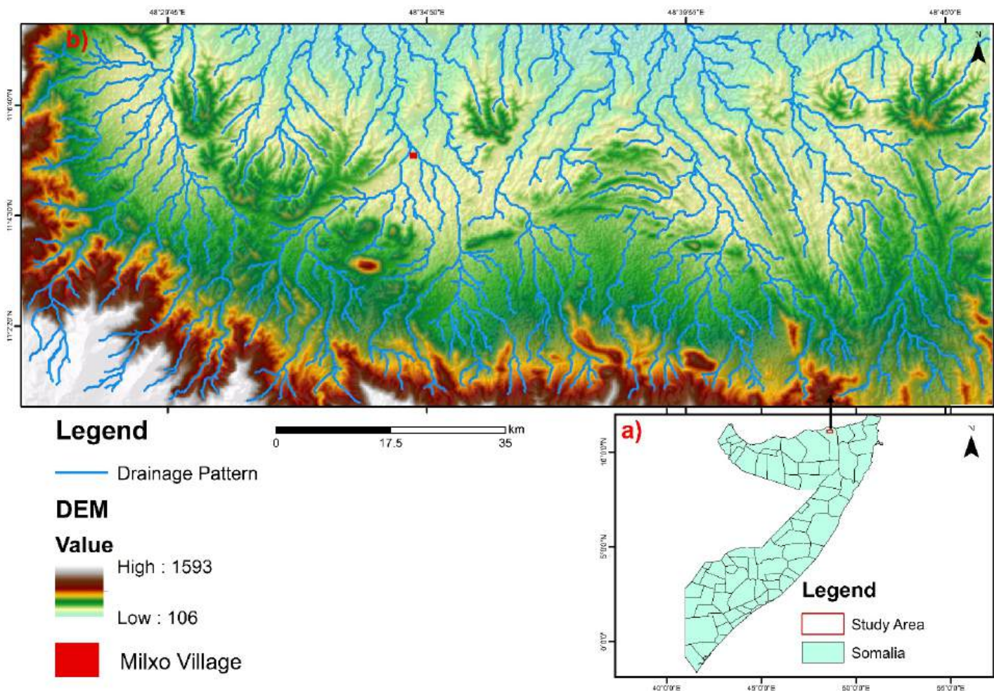
Fig. 1 (a) Geographical location of Somalia; (b) study area, Milxo Village, northern Somalia.
